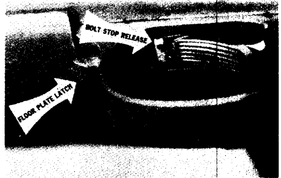
Figure 2-2. Bolt Stop Release and Floor Plate Latch.
